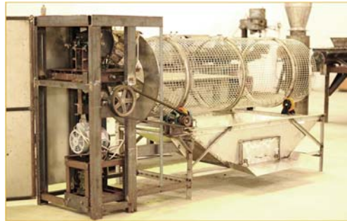
Figure 1 Cocoa bean separator from cocoa pod.
