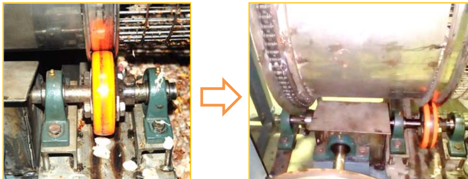
Figure 5 An improvement of the transmission system from a friction drive to a chain drive.
