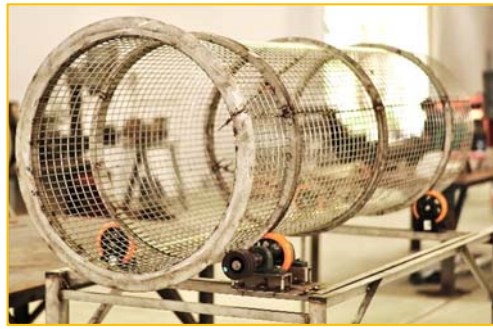
Figure 3 Cylinder sieve separates cocoa beans by rotation.
