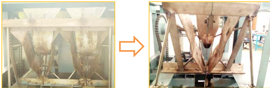
Figure 4 An improvement of the v-shaped input box from 2 and wider boxes to 1 and narrower box.
